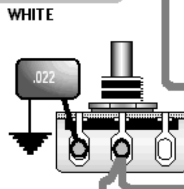
MASTER TONE POT 250K AUDIO TAPER
