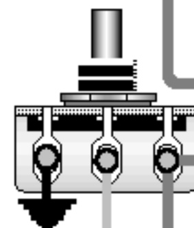
VOLUME POT 250K AUDIO TAPER
